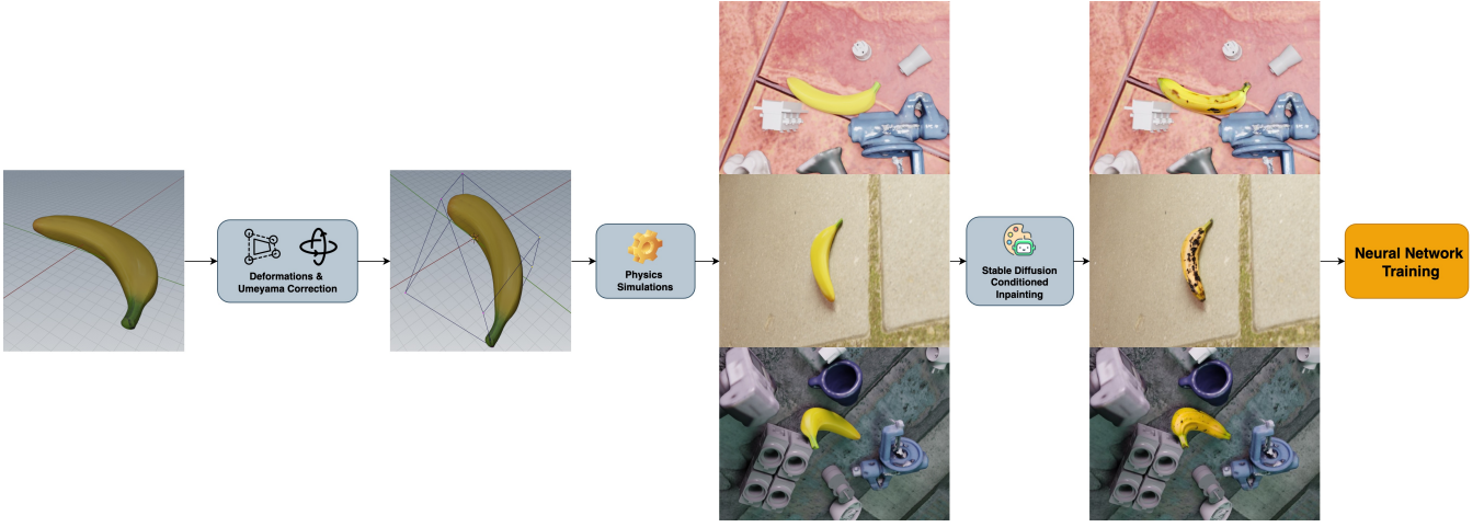
Fig. 2: Overview of the PLANTPose framework. Given a base mesh, we generate deformed object instances using lattice-based deformations. These instances are placed in physically plausible synthetic scenes rendered in Blender, which are further refined using Stable Diffusion inpainting to enhance texture realism. The generated dataset is then used to train a deep learning model for simultaneous 6D pose estimation and deformation prediction.
