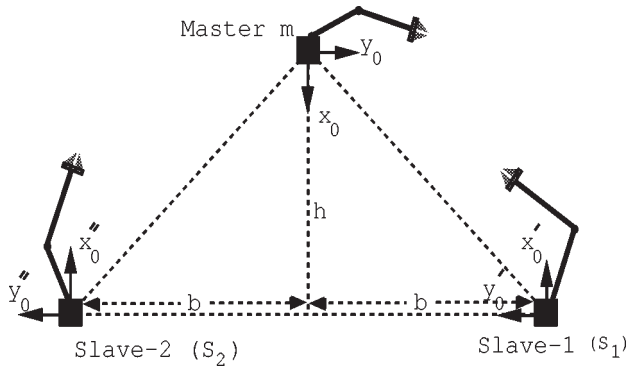
Figure 1. Symmetric master-and-two-slaves configuration (all axes z_0, z'_0, z''_0 are normal to the plane m - s_1 - s_2 ).
