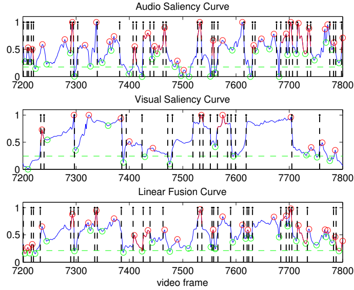
Fig. 1.8. Curves and detected features for audio saliency (top), video saliency (middle) and audiovisual saliency (bottom). The frame sequence was from the movie “Lord of the Rings I”.
