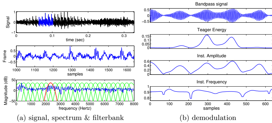
Fig. 1.1. Short-time audio processing and dominant modulation extraction. (a) a vowel frame (20ms) from a speech waveform is analyzed in multiple bands (bottom) and (b) the dominant, w.r.t average source energy, band is demodulated in instantaneous amplitude and frequency (smoothed by 13-pt median) signals.
