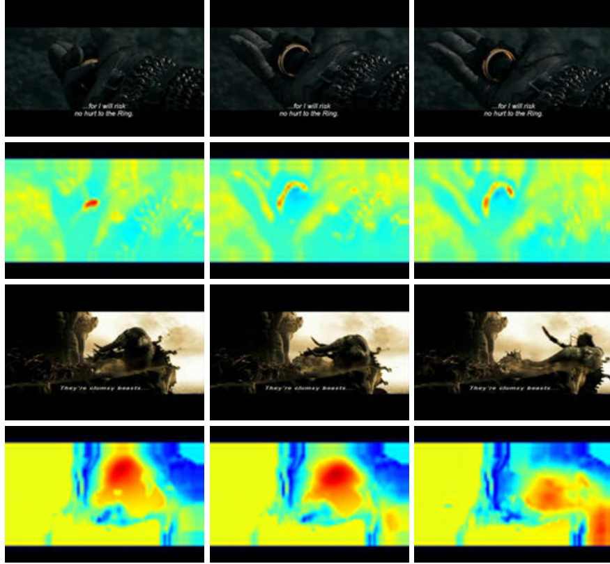
Fig. 1.5. Original frames from the movies “Lord of the Rings I” (top) and “300” (bottom) and the corresponding saliency maps (better viewed in color).
