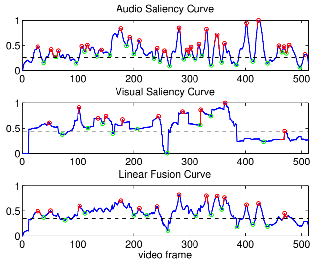
Fig. 1.6. Saliency curves and detected features (maxima, minima, lobes and levels) for audio (top), video (middle) and audiovisual streams (bottom) of the movie trailer “First Descend”.
