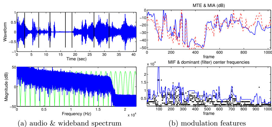
Fig. 1.2. Feature extraction from multi-source audio stream. (a) Waveform with manual labeling of the various sources/events (vertical lines) and wideband spectrum with filterbank, (b) top: MTE (solid) and MIA (dashed), bottom: MIF with dominant carrier frequencies superimposed (1024 frames from “300” video).
