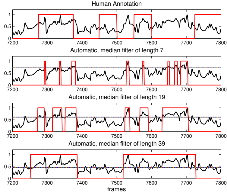
Fig. 1.9. Human and automated saliency-based annotations. Top row: Audiovisual saliency curve and manual annotation by inspection superimposed. Saliency indicator functions obtained with a median filter of variable size (7, 19, 39) in all other plots. The frame sequence was the same as in Fig. 1.8.
