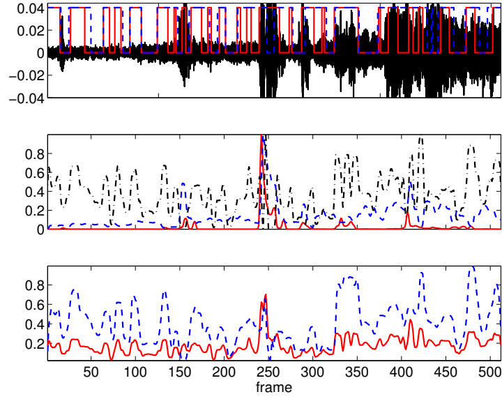
Fig. 1.3. Audio saliency curves. Top: audio waveform and threshold-based saliency indicator functions, Middle: normalized audio features, MTE (solid), MIA (dashed), MIF (dash dotted). Bottom: saliency curve (linear in solid, nonlinear in dashed). Indicator functions correspond to the two audio fusion schemes, (512 frames from the “Lord of the Rings I” stream).
